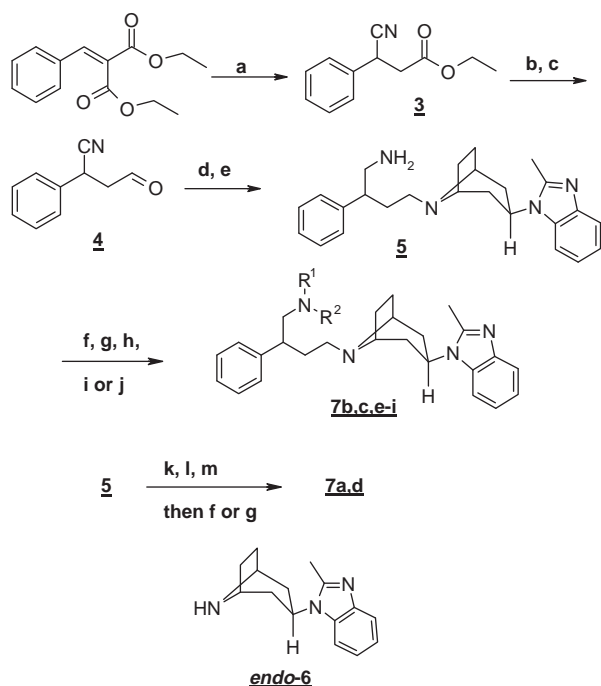
Scheme 1. Reagents and conditions: (a) KCN, EtOH–H 2 O, 70 °C, overnight, 73%; (b) LiBH 4 , THF, reflux, 2 h, 59%; (c) Dess–Martin periodinane, CH 2 Cl 2 , rt, 2 h, 89%; (d) NaBH(OAc) 3 , endo-6 , CH 2 Cl 2 , rt, 18 h, 70%; (e) Raney–Ni, H 2 (50 psi), EtOH/concd NH 4 OH (6:1), rt, 18 h, 99%; (f) 4,4-difluorocyclohexanecarboxylic acid, HATU, iPr 2 NEt, CH 2 Cl 2 , rt, 2 h, 56%; (g) RSO 2 Cl, iPr 2 NEt, CH 2 Cl 2 , rt, 37–74%; (h) morpholine-4-sulfonyl chloride, ACN, iPr 2 NEt, 5 h, 80 °C, 70–72%; (i) Ac 2 O, iPr 2 NEt, CH 2 Cl 2 , rt, 83%; (j) iPr 2 NEt, P(O)(OMe) 2 Cl, CH 2 Cl 2 , rt, 43%; (k) o -NosCl, iPr 2 NEt, CH 2 Cl 2 , 74%; (l) (i) NaH, THF, rt; (ii) MeI, 80%; (m) LiOH, HSCH 2 CO 2 H, DMF, rt, 2 h, 100%.
