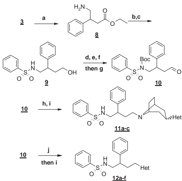
Scheme 2. Reagents and conditions: (a) Pd/C, H 2 (60 psi), EtOH, concd HCl, rt, overnight, 45%; (b) PhSO 2 Cl, iPr 2 NEt, CH 2 Cl 2 , rt, 18 h, 92%; (c) LiBH 4 , THF, 65 °C, 2 h, 100%; (d) TBSCl, DMAP, ImH, CH 2 Cl 2 , 30 min, rt, 88%; (e) (i) DMF, NaH; (ii) Boc 2 O, rt, 1 h, 55%; (f) THF, TBAF, AcOH, rt, 18 h, 100%; (g) DMP, CH 2 Cl 2 , 2 h, rt, 82%; (h) tropanes corresponding to entries 11a–c in Table 2, NaBH(OAc) 3 , CH 2 Cl 2 , rt; (i) TFA, CH 2 Cl 2 , rt, 3 h; (j) amines corresponding to entries 12a–f in Table 2, NaBH(OAc) 3 , CH 2 Cl 2 , rt.
