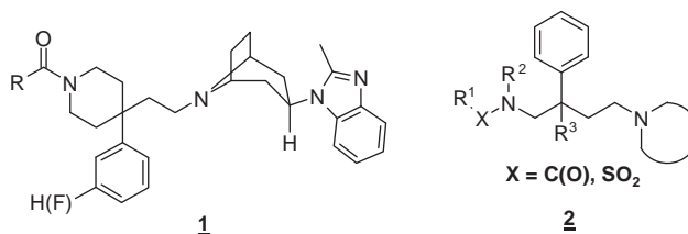
Figure 1. 4,4-Disubstituted piperidine 1 and diaminobutane (DAB) scaffold 2 .
