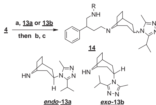
Scheme 3. Reagents and conditions: (a) NaBH(OAc) 3 , CH 2 Cl 2 , rt, 18 h, 93%; (b) Raney–Ni, H 2 (60 psi), EtOH, concd NH 4 OH, rt, 18 h, 95%; (c) RCO 2 H/HATU/iPr 2 NEt/CH 2 Cl 2 or RSO 2 Cl/iPr 2 NEt/CH 2 Cl 2 , rt, 1–2 h.
