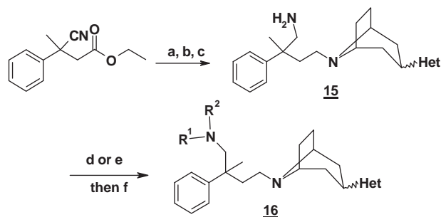
Scheme 4. Reagents and conditions: (a) DIBAL-H, THF, -78^{\circ}\text{C} , 1 h, 19%; (b) \text{NaBH}(\text{OAc})_3 , 5 or 13b , \text{CH}_2\text{Cl}_2 , rt, 18 h; 85%; (c) Raney-Ni, \text{H}_2 (50 psi), EtOH, concd \text{NH}_4\text{OH} , 50^{\circ}\text{C} , 18 h, 90%; (d) HATU, difluorocyclohexylcarboxylic acid, i\text{Pr}_2\text{NEt} , \text{CH}_2\text{Cl}_2 , rt, 18 h, 72%; (e) \text{PhSO}_2\text{Cl} , i\text{Pr}_2\text{NEt} , \text{CH}_2\text{Cl}_2 , rt, 18 h, 73%; (f) NaH, THF or DMF then MeI, 7–75%.
